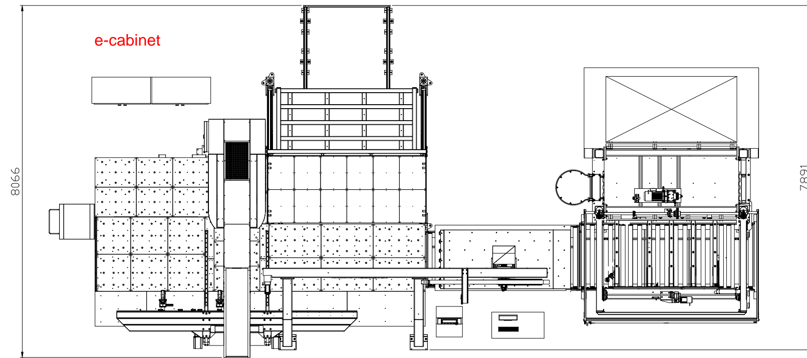
CNC Turret Punch
